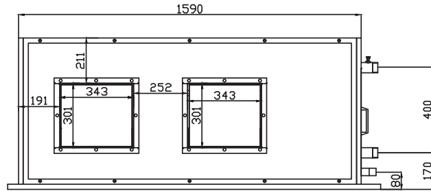
Vista Frontal
