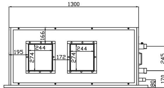
Vista Frontal
